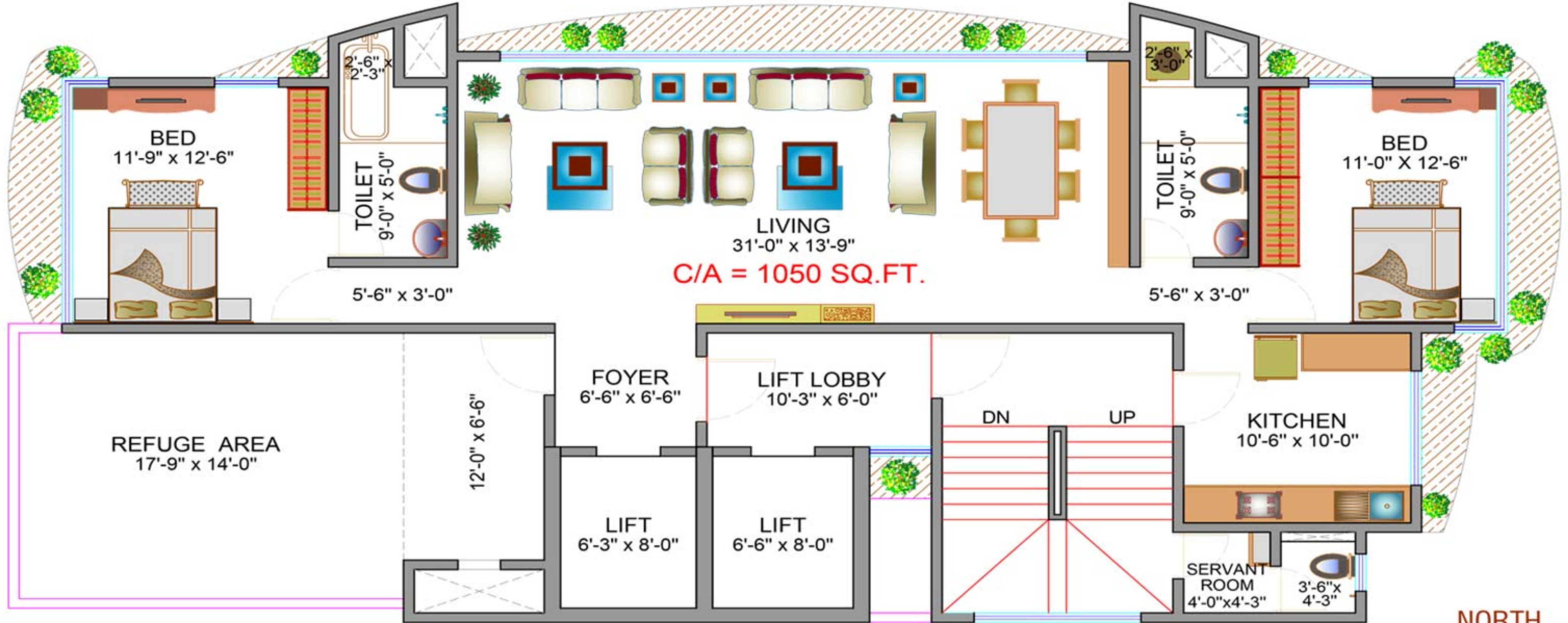
6TH FLOOR PLAN (REFUGE)
